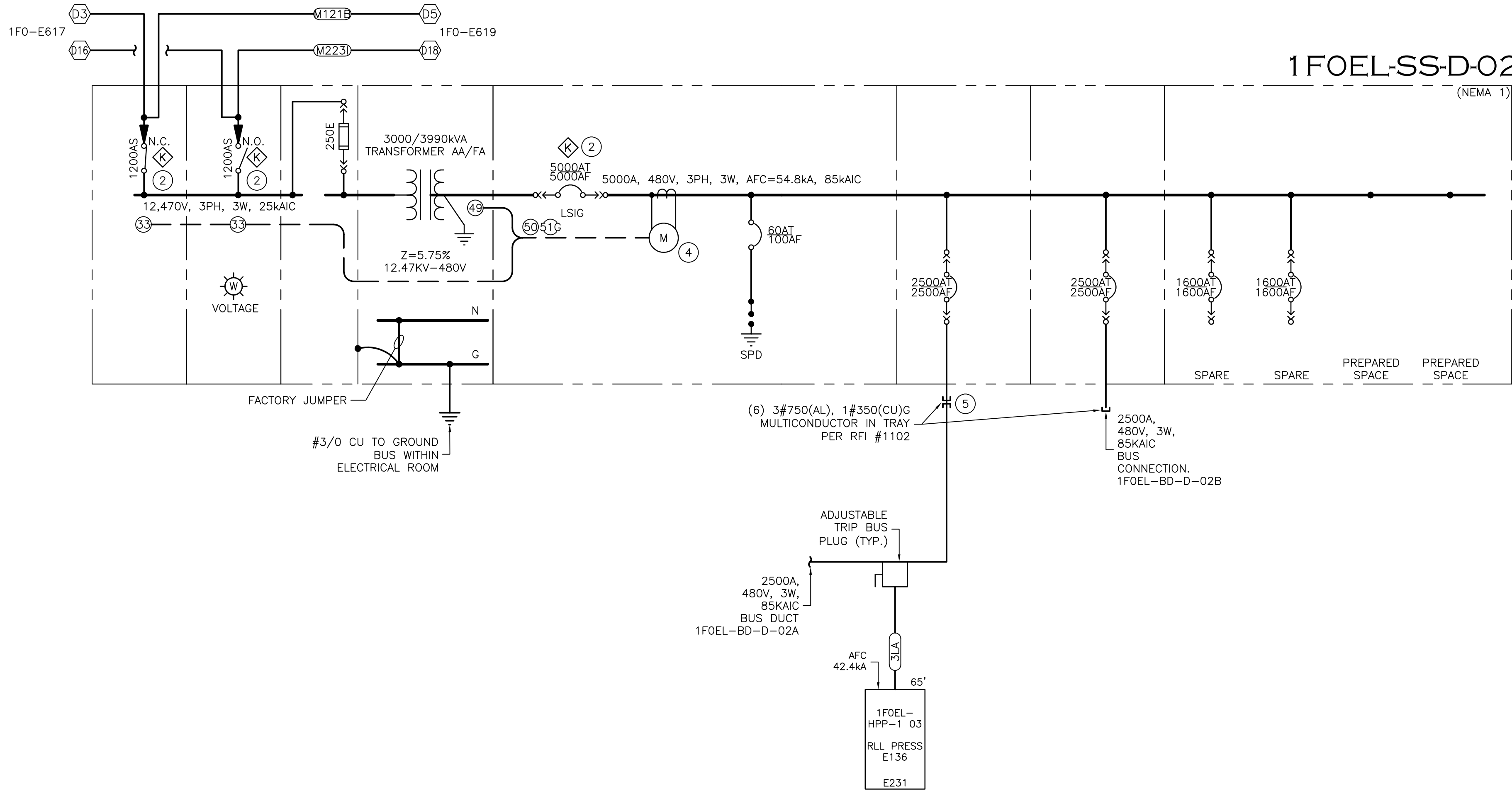
ONE LINE DIAGRAM - (1FO) ELECTRODE "D" (PARTIAL) NO SCALE
